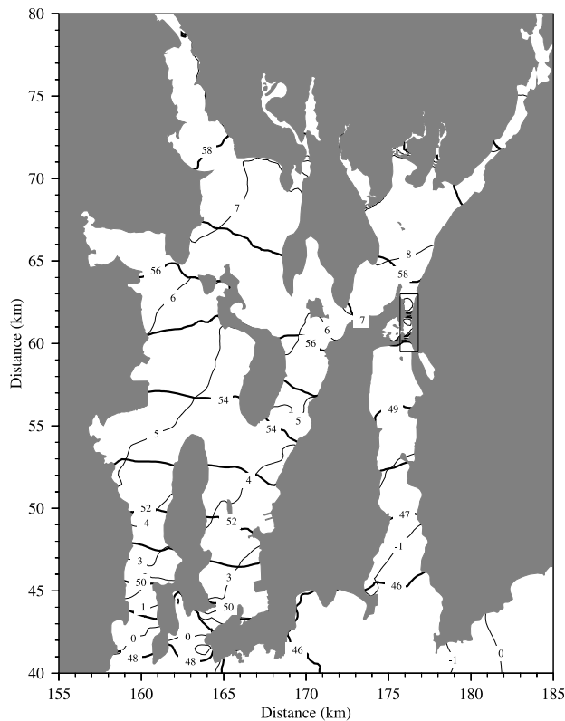
Figure 3. Co-tidal chart of the model-predicted M_2 tidal elevation. Heavy solid line: Co-amplitude (cm) and thin solid line: co-phase ( ^{\circ}\text{G} ).
