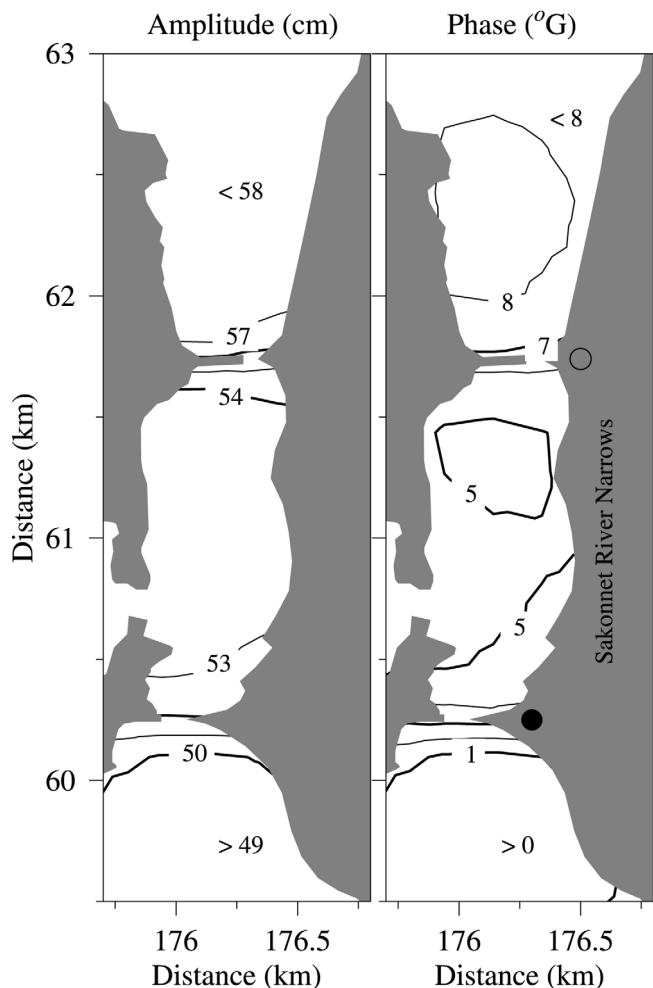
Figure 4. Co-amplitudes (cm) (left) and co-phases ( ^{\circ}\text{G} ) (right) of the M_2 tidal elevation in the MHB-SR channel. Open circle, the Sakonnet River Bridge; solid circle, the Stone Bridge.
