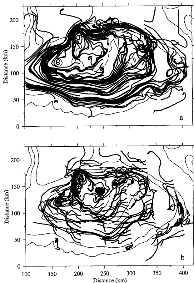
Fig. 9. The near-surface (a) and near-bottom (b) trajectories of particles over Georges Bank for the case with tide only forcing and the temperature and salinity fields shown in Fig. 6. Each dot indicates the initial location of a particle. The particles were released in the July–August stratified flow field at the end of the 10th model day and followed for 30 days.
