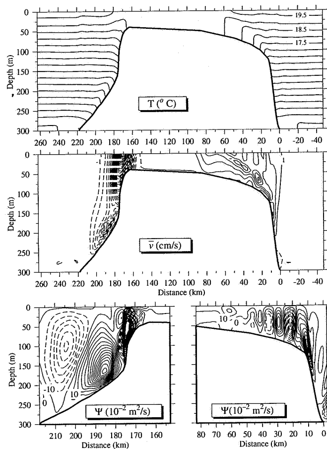
Fig. 5. Cross-bank distributions of tidally-averaged temperature, along-bank velocity, and cross-bank streamfunction. The direction of the along-bank residual current (middle panel): positive-out of the page; negative: into the page. The direction of the cross-bank residual current (lower panel) is defined as \bar{u} = -\partial\Psi/\partial z ; \bar{w} = \partial\Psi/\partial x .
