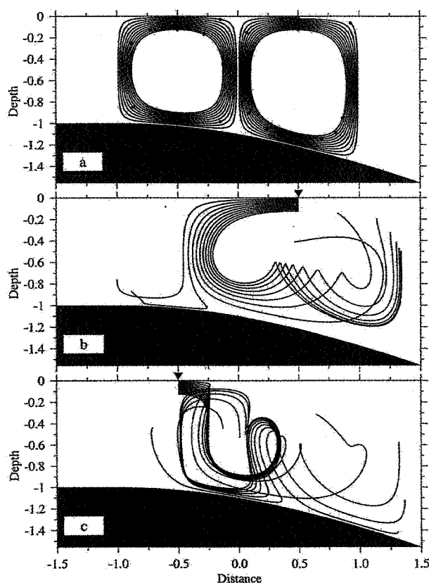
Fig. 16. Trajectories of 20 particles released near the surface at the center of the circulation cells for the cases in which the double cells were steady (a) and oscillated with a period of 14 days (b) and (c). In both the cases, \psi_0 = 0.35 \text{ m}^2/\text{s} and L = 5 \text{ km} . In the oscillatory case, a_0 = 2.5 \text{ km} . The open circles and filled dots in (a) are the initial and ending positions of particles. The filled downtriangle in (b) and (c) indicates the starting location of particles. The cross-shelf distance and vertical depth were scaled by 5 km and 40 m.
