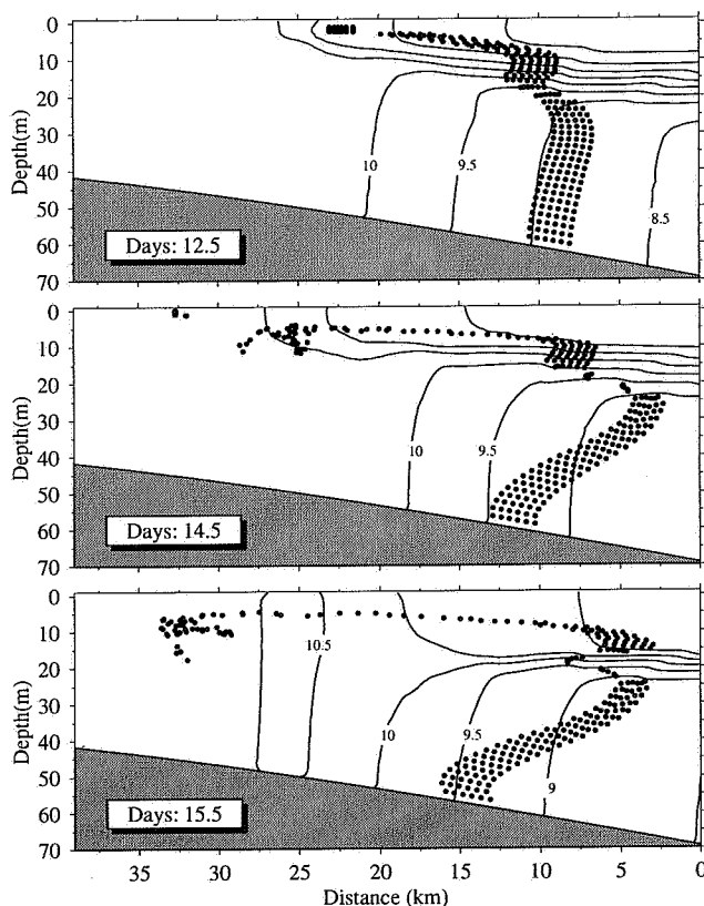
Fig. 15. Distribution of particles at the 12.5th (upper), 14.5th (middle), and 15.5th (lower) model days for the case with tidal forcing plus realistic wind. The contours are the model-predicted temperatures.
