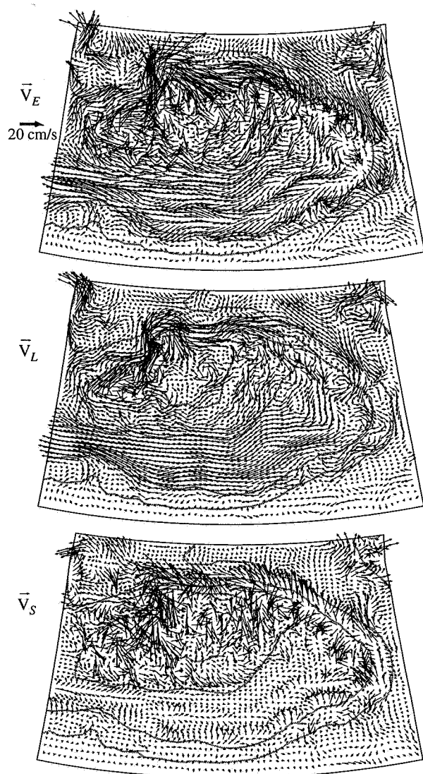
Fig. 7. Distributions of the near-surface residual Eulerian ( \bar{V}_E ), Lagrangian ( \bar{V}_L ), and Stokes' ( \bar{V}_S ) velocities for the case with temperature and salinity fields shown in Fig. 6.
