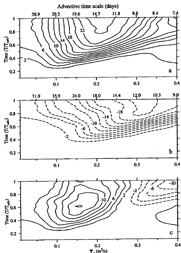
Fig. 17. The distribution of the percent of the cross-cell particles with respect to the amplitude of the cell circulation ( \psi_0 ) and the non-dimensional time scaled by the advective time scale ( T/T_{adv} ) for the sloping-bottom case (a: seaward-from the left cell to the right cell; b: onshore-from the right cell to the left cell). The digital number at the top of (a) and (b) indicates the advective time scale (days) for a given \psi_0 .
