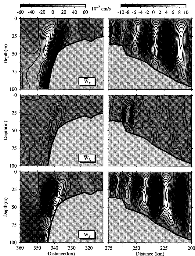
Fig. 8. Cross-bank distributions of the residual Eulerian ( \bar{W}_E ), Lagrangian ( \bar{W}_L ), and Stokes' ( \bar{W}_S ) vertical velocities for the case with temperature and salinity fields shown in Fig. 6.
