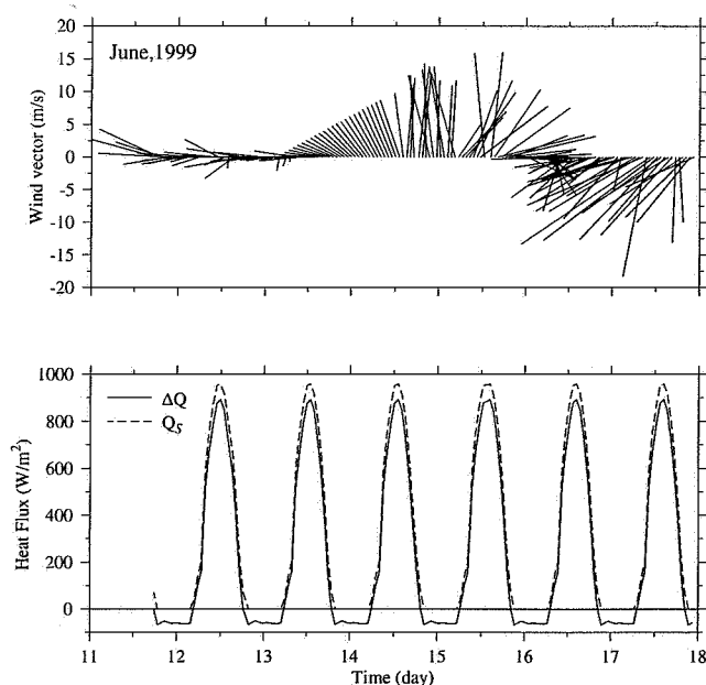
Fig. 13. Time series of the surface wind velocity vectors and heat flux on the southern flank of Georges Bank. The wind data was obtained from the June 1999 cruise around the tidal mixing front on the southern flank of the center Georges Bank, and the heat flux data came from the 1995 meteorological buoy measurement on the southern flank. \Delta Q and Q_s are the net surface heat flux and shortwave radiation, respectively.
