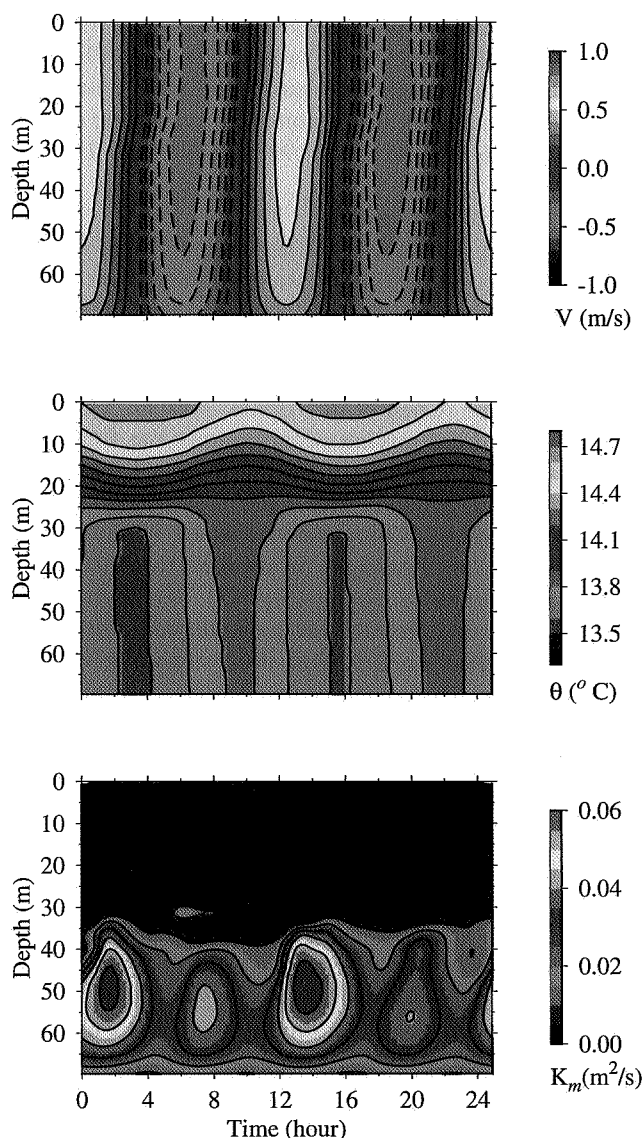
Fig. 12. Model-predicted time series of cross-bank current ( V ), temperature ( \theta ), vertical thermal and diffusion coefficient ( K_m ) at a selected site around the 60-m isobath on the center of Georges Bank. This figure is replotted based on figure 16 in Chen et al. (2001a).
