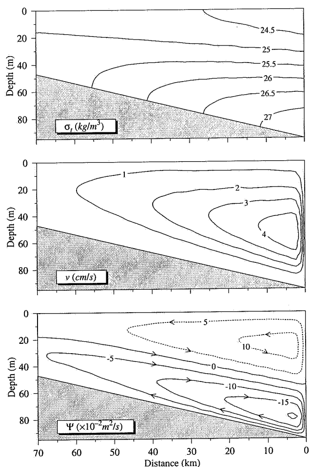
Fig. 4. Distributions of density, along-isobath current and cross-isobath streamfunction calculated using the semi-analytical, diagnostic frontal model.
