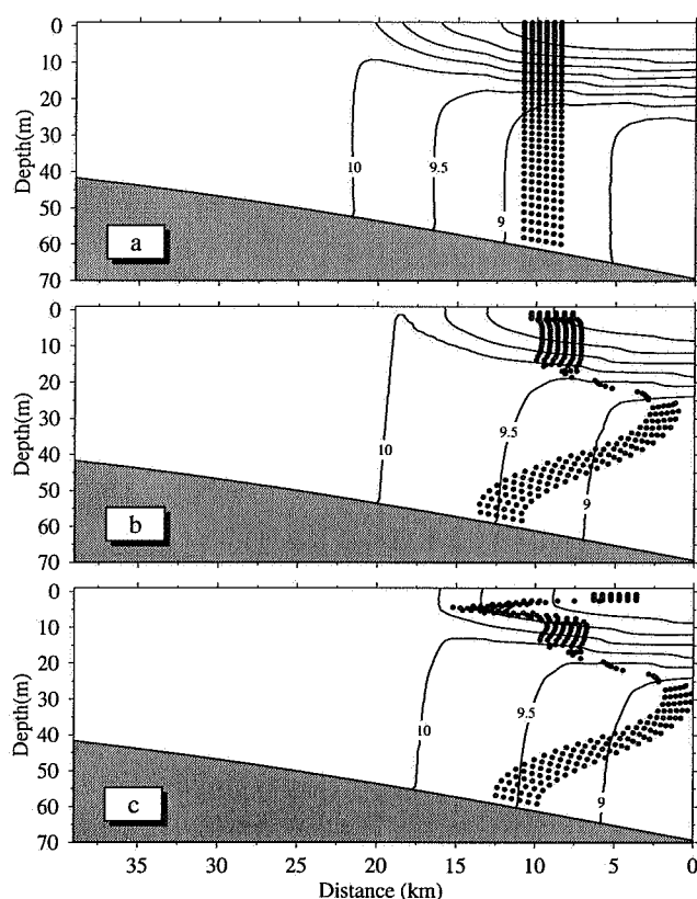
Fig. 14. Distribution of particles at the initial (the 11th model day) (upper) and at the 15.5th model day for the cases with tidal forcing only (middle) and with tidal forcing plus mean wind (lower). The contours are the model-predicted temperatures
