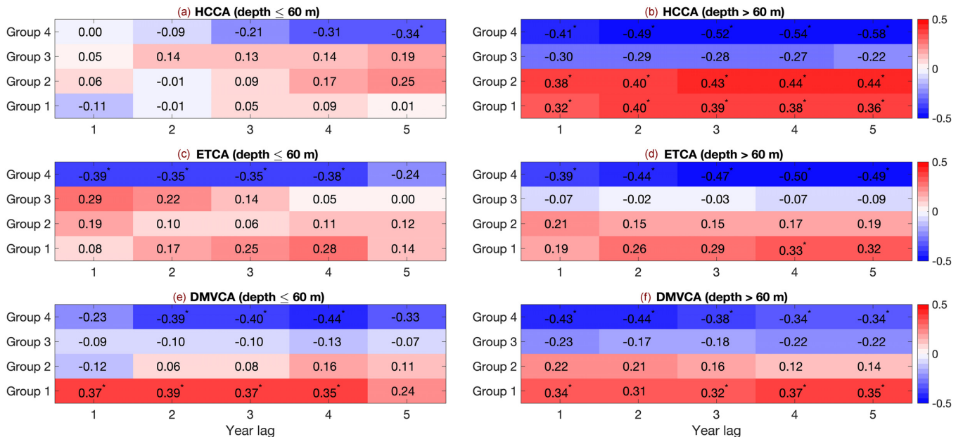
Figure 7. Left panels are the interannual correlations between the percentages of SOM groups and thermal stress (i.e. number of days with bottom temperature > 13^{\circ}\text{C} ) in shallow closed areas with bottom depth \leq 60 m (a: HCCA; c: ETCA; e: DMVCA). Right panels are the interannual correlations between the percentages of SOM groups and fishing mortality in deep closed areas with bottom depth > 60 m (b: HCCA; d: ETCA; f: DMVCA). X axis in each panel represents 1–5 years' running average (*: P value < 0.05 ).
