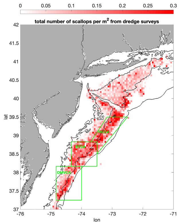
Figure 1. The climatology of Atlantic sea scallop density in the MAB from 1978 to 2017 (data source: dredge survey data provided by NOAA). The three black contour lines represent 35, 60, and 100 m isobaths, respectively. The three green boxes are the rotationally closed areas (HCCA: Hudson Canyon South Closed Area; ETCA: Elephant Trunk Closed Area; DMVCA: Delmarva Closed Area).
