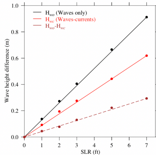
Fig. 19 Changes of the significant wave height difference (relative to the value for the case without SLR) with SLR over the Winthrop Peninsula coast under the conditions without and with the inclusion of wave-current interactions.
