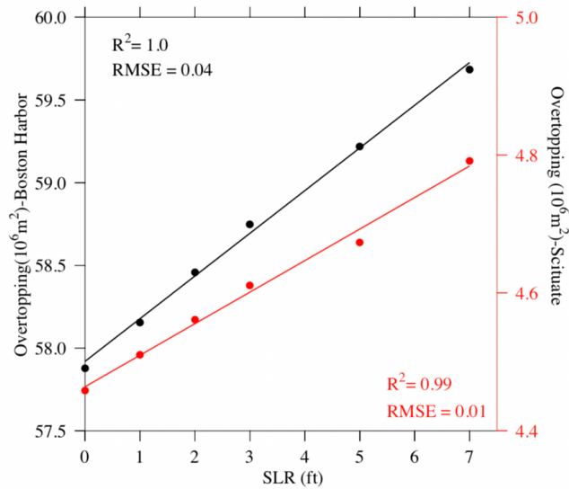
Fig. 17 Changes of overtopping with SLR over the coasts of Boston and Scituate Harbors, respectively. Black: Boston Harbor; red: Scituate Harbor.
