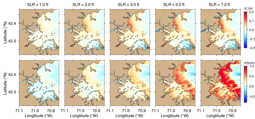
Fig. 11 Differences of the surface elevation ( \Delta\zeta ) and significant wave height ( \Delta H_s ) relative to \zeta and H_s from the case with SLR = 0.0 for the cases with SLR of 1, 2, 3, 5, and 7 ft in Boston Harbor.
