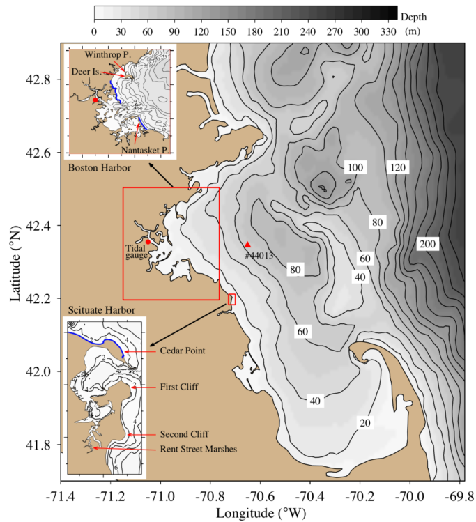
Fig. 1 Bathymetry of Mass Bay (MB) with enlarged views in Boston and Scituate Harbors. Blue curvature lines in enlarged left up and low panels are the coasts where the wave run-up overtopping is calculated. The red filled triangle is the location of NOAA Buoy#44013. The red filled dot is the location of the tidal gauge.
