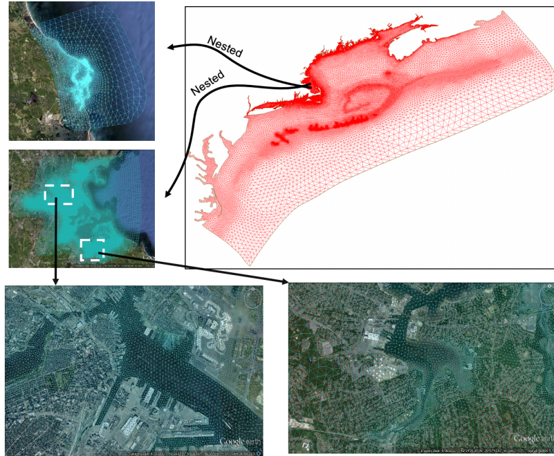
Fig. 3 The horizontal FVCOM grids of Scituate and Boston Harbors nested with the NECOFS regional FVCOM model. An example of an enlarged view of the model grid over the land and rivers is given in the lower panel. The horizontal resolution is up to ~10 m inside harbors and over the land.
