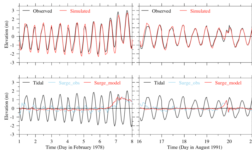
Fig 6 Comparisons of the observed and simulated total (upper) and storm surge (lower) elevations at the tidal gauge site in Boston Harbor over February 1-8, 1978 (left), and August 16-21, 1991 (right).
