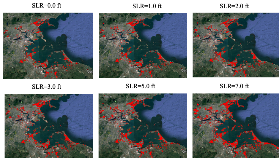
Fig. 13 Inundation maps over the Boston Harbor's coast for the cases with SLR of 1, 2, 3, 5, and 7 ft, respectively.
