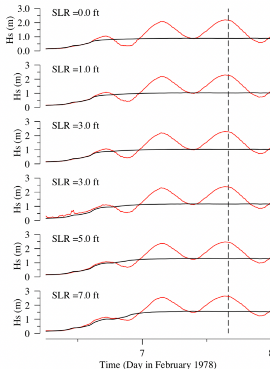
Fig. 18 Changes of the significant wave height with SLR over the Winthrop Peninsula coast under the conditions without and with the inclusion of wave-current interactions.
