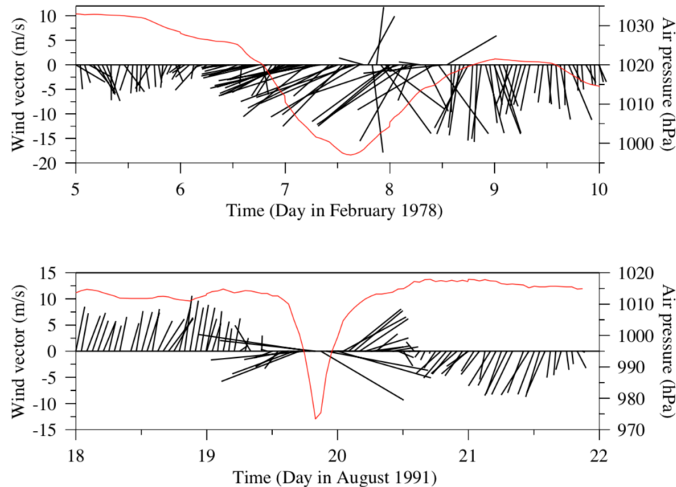
Fig. 5 Time series of wind vector and air pressure (red line) at NOAA Buoy#44013 over February 5-10, 1978 (based on the model prediction) and August 18-22, 1991 (based on the measurement records).
