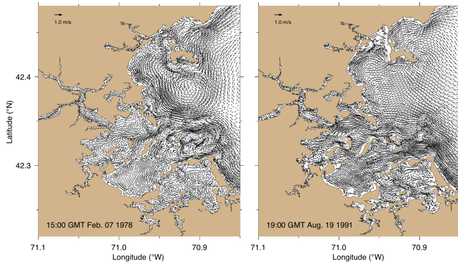
Fig. 9 Distributions of near-surface water velocities in Boston Harbor at 15: 00 GMT, February 7, and 19:00 GMT, August 19, 1991, respectively.
