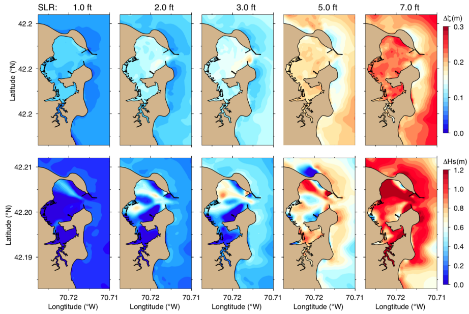
Fig. 12 Differences of the surface elevation ( \Delta\zeta ) and significant wave height ( \Delta H_s ) relative to \zeta and H_s from the case with SLR = 0.0 for the cases with SLR of 1, 2, 3 5, and 7 ft in Scituate Harbor, respectively.
