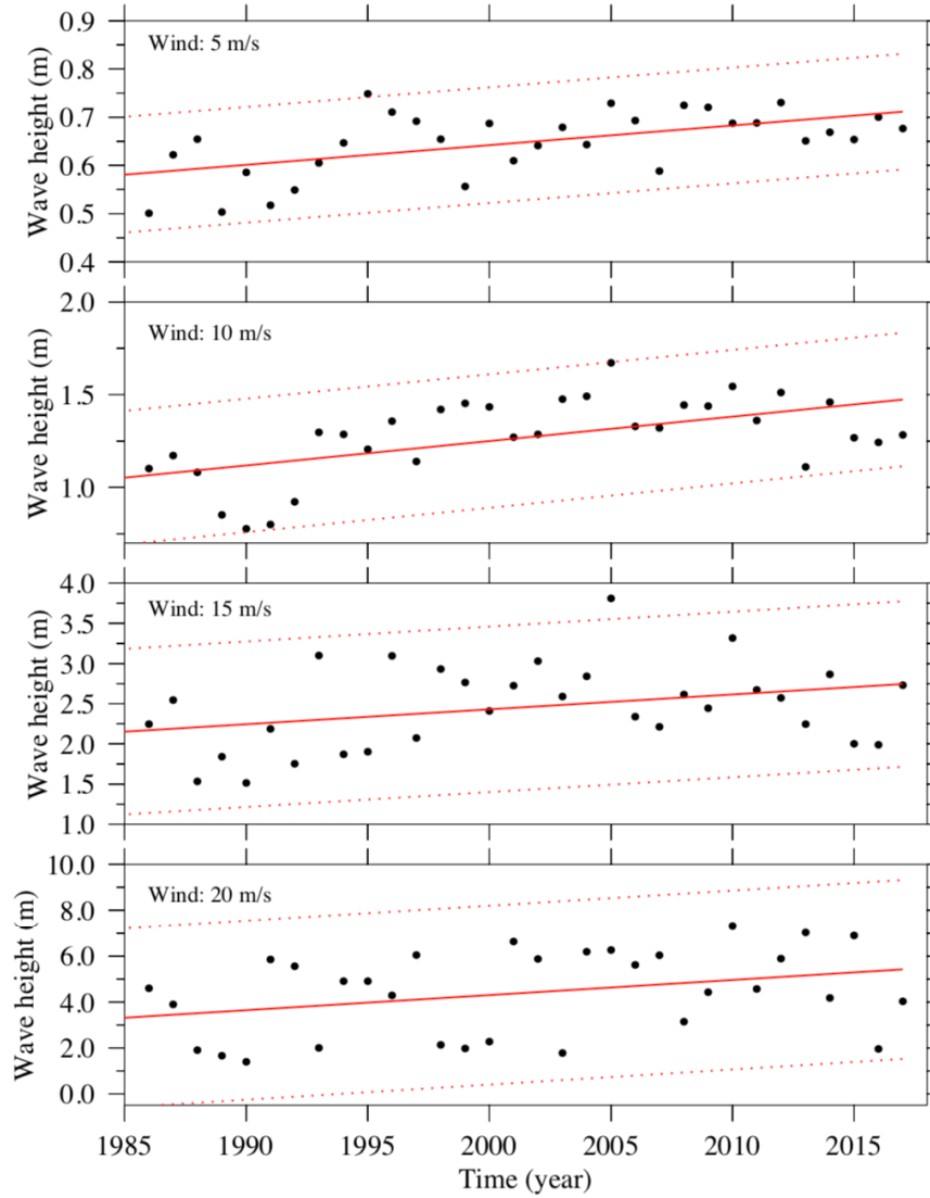
Fig. 20 Interannual variability of the significant wave height under given wind speeds of 5, 10, 15, and 20 m/s over 1985-2017, respectively.
