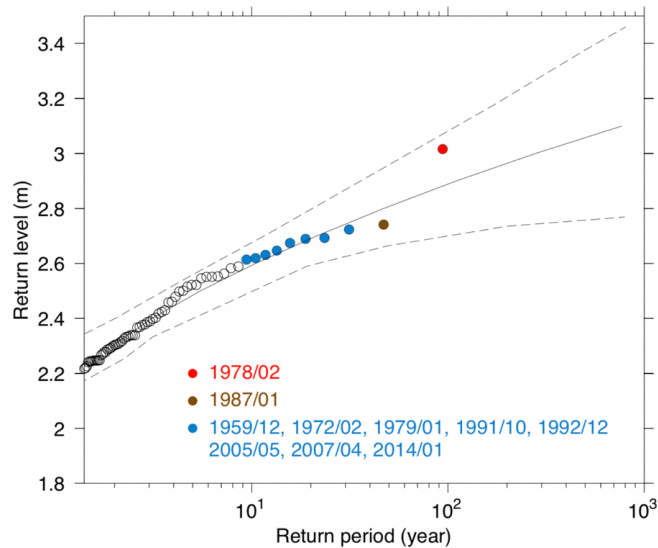
Fig. 4 Storm return high water level versus return period summarized from the data recording at NOAA Buoy#44013 and tidal gauge in Boston Harbor before 2015.
