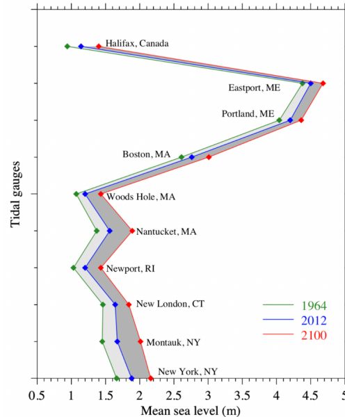
Fig. 2 Projected mean sea level rise over the New England coast from New York on the south to Halifax. The figure was drawn based on the projection of the mean sea level at tidal gauges.
