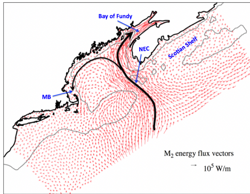
Fig. 21 Map of the M_2 tidal energy flux vectors in the Gulf of Maine predicted by the NECOFS. MB: Mass Bay, NEC: Northeast Channel.
