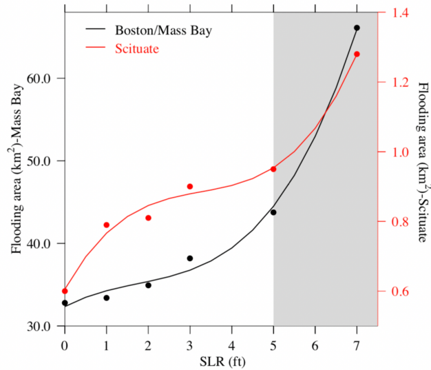
Fig. 15 Changes in the flooding area with SLR over the coasts of Boston and Scituate Harbors. Note: the wave runup-produced overtopping is not taken into account.
