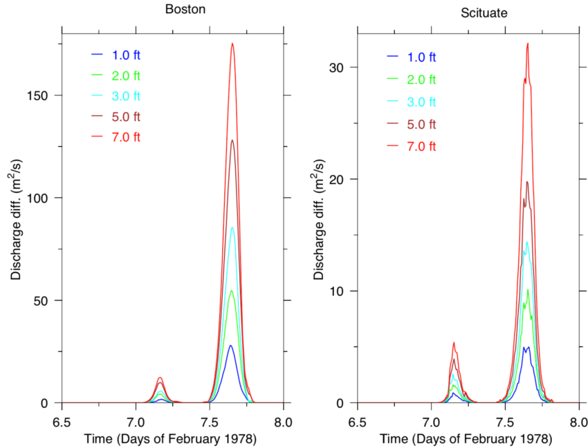
Fig. 16 Differences of the overtopping discharge relative to the value for the case with SLR = 0.0 for the cases with SLR of 1, 2, 3, 5, and 7 ft. Left: Boston Harbor, right: Scituate Harbor.
