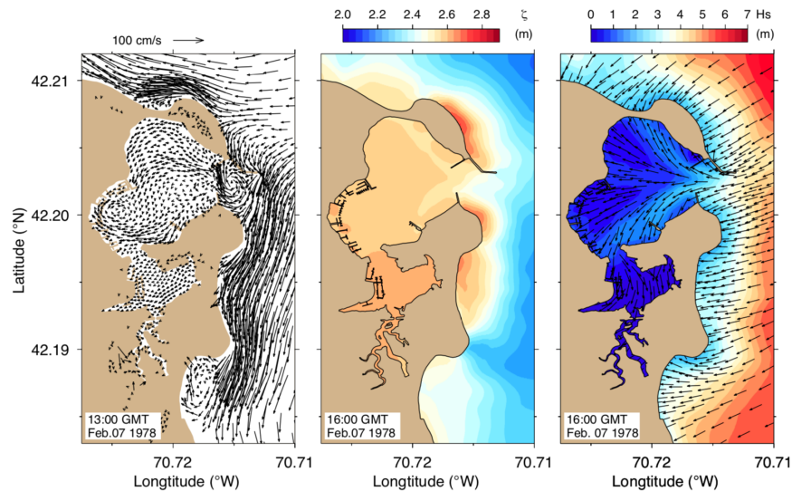
Fig. 10 Distributions of the near-surface water velocity (left) at 13:00 GMT, surface elevation (middle), and significant wave height (right) at 16:00 GMT, February 7, 1978, in Scituate Harbor.
