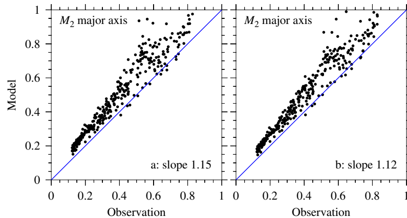
Fig. 22. Scatter plots of the CODAR-derived and model-computed major axes of the M_2 tidal current (m/s): (a) for the case with the updated bathymetry; (b) for the case with an increased bottom roughness. The blue line with a slope of 1 has been added for reference. The slope of the least-squares linear fit to the data is shown in the lower right of each panel. (For interpretation of the references to color in this figure legend, the reader is referred to the web version of this article.)
