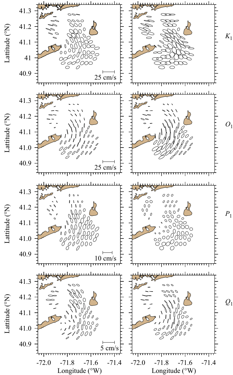
Fig. 5b. CODAR-derived (left panels) and FVCOM-computed (right panels) diurnal tidal current ellipses for K_1 , O_1 , P_1 and Q_1 .
