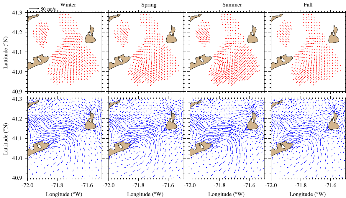
Fig. 9. Comparisons of CODAR-derived (upper panels) and model-computed (lower panels) mean surface currents in winter, spring, summer and fall averaged seasonally over 2000–2008 (using only data from the ‘system on’ periods). Red arrows: CODAR-derived at the selected grid points; blue arrows: model-computed. (For interpretation of the references to color in this figure legend, the reader is referred to the web version of this article.)
