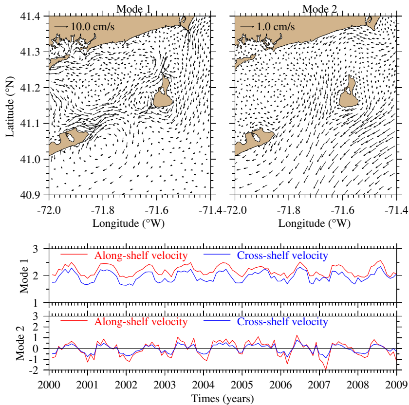
Fig. 18. The two Empirical Orthogonal Function (EOF) modes dominating the flow field in Block Island Sound based on an analysis of the nine-year NECOFS vertically-averaged flow field. Upper panel: spatial distributions of the vertically-averaged velocity for the first two EOF modes. Lower panel: the associated temporal amplitudes of the along and cross shelf velocities associated with the 1st and 2nd EOF modes.
