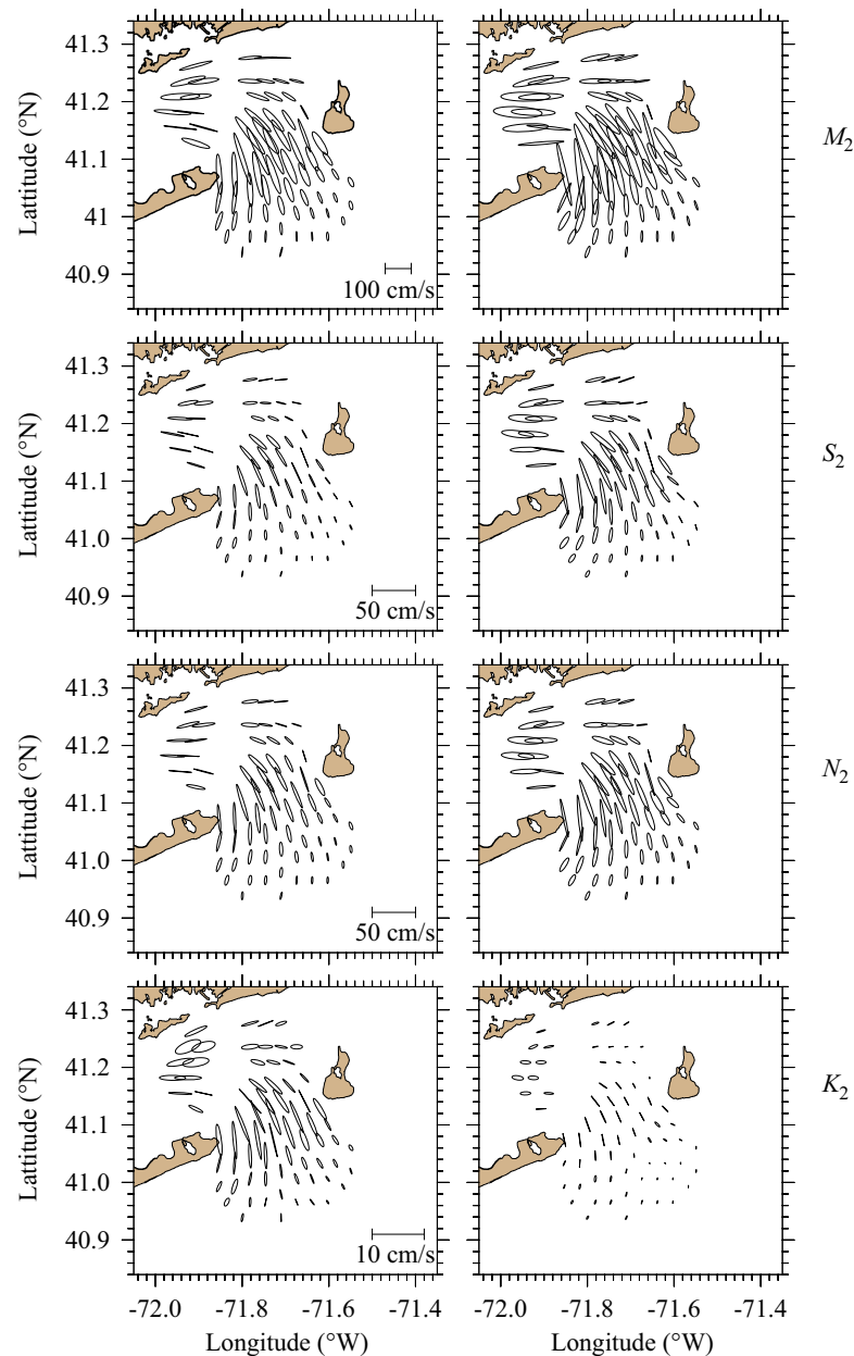
Fig. 5a. Comparisons of NECOFS-computed and CODAR-derived semi-diurnal tidal current ellipses for M_2 , S_2 , N_2 and K_2 . Left panels: CODAR-derived and right panels: FVCOM-computed.
