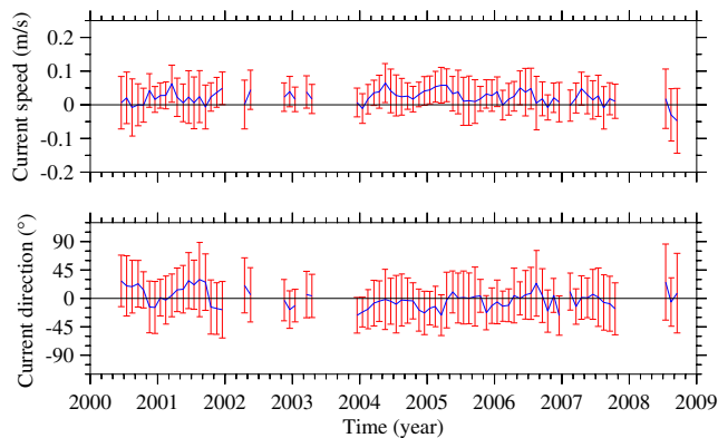
Fig. 10. The difference (blue line) and standard deviation (red line) in magnitudes (upper panel) and directions (lower panel) of the 75 model-computed and CODAR-derived monthly surface velocities averaged over the 334 selected grid points from 2000 to 2008. (For interpretation of the references to color in this figure legend, the reader is referred to the web version of this article.)
