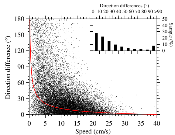
Fig. 11. The larger panel shows scatter plots of the difference for the CODAR-derived and model-computed direction; the red curve is calculated from Lowess curve fitting. The upper panel shows the percentage for difference in direction. (For interpretation of the references to color in this figure legend, the reader is referred to the web version of this article.)
