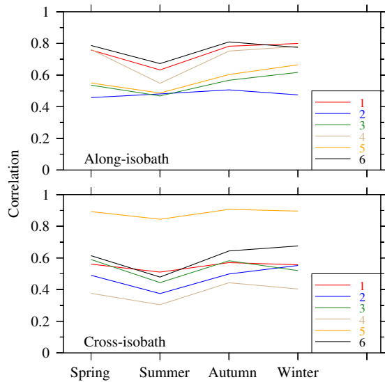
Fig. 20. Seasonal variability of the maximum wind-current correlation coefficient at sites 1–6, the along-isobath velocity in upper panel and the cross-isobath velocity in lower panel. The correlation coefficient is a seasonally-averaged value over the period 2000–2008.
