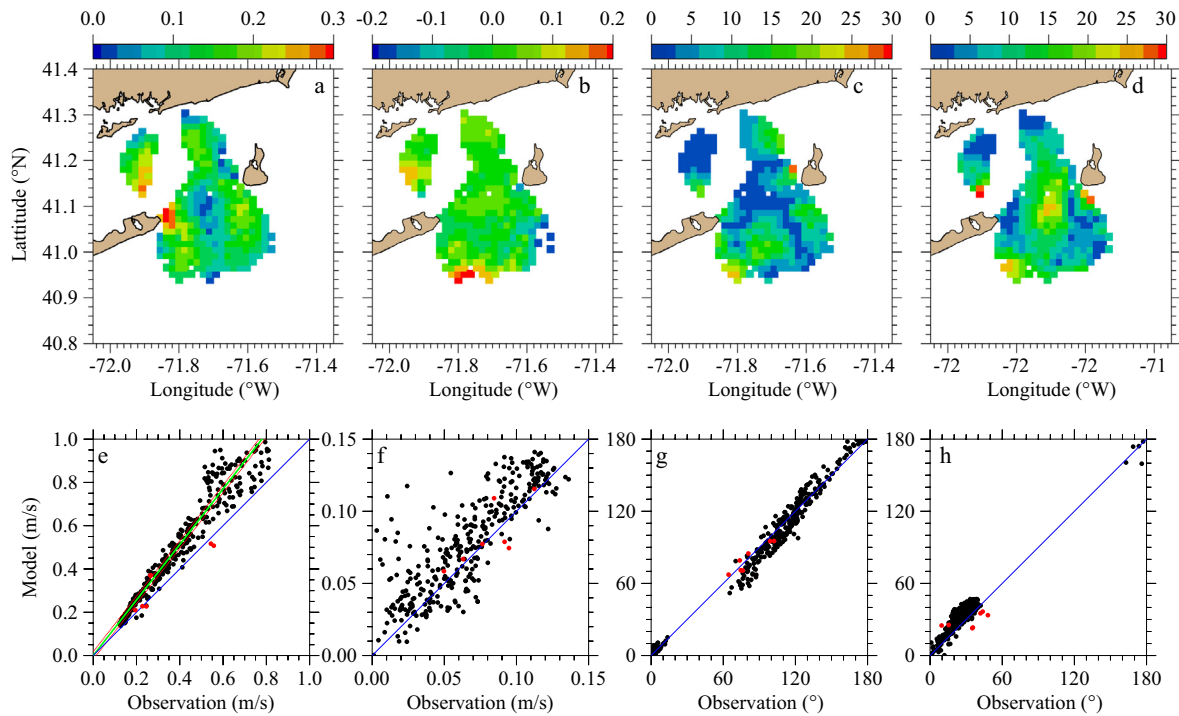
Fig. 6. Upper row: distributions of differences in (a) normalized major axis, (b) eccentricity, (c) orientation ( ^{\circ} ) and (d) phase ( ^{\circ} ) calculated based on CODAR-derived and model-computed M^2 tidal currents; lower row: scatter plots (black dots) of the CODAR-derived and model-computed (e) major axis (m/s), (f) minor axis (m/s), (g) orientation ( ^{\circ} ) and (h) phase ( ^{\circ} ) between model and CODAR (black dots). The blue line with a slope of 1 has been added in panel (e) for reference. The green line in panel (e) is the least-square fit of y = a + bx . Also shown are scatter plots (red dots) of the vertical-averaged ADCP-derived and model-computed ellipse parameters. (For interpretation of the references to color in this figure legend, the reader is referred to the web version of this article.)
