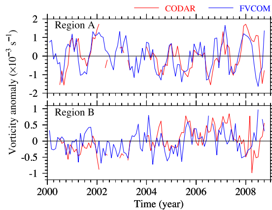
Fig. 13. Comparisons of the time series of vorticity anomalies calculated from the CODAR-derived and model-computed surface velocity fields in Region A (upper panel) and Region B (lower panel).
