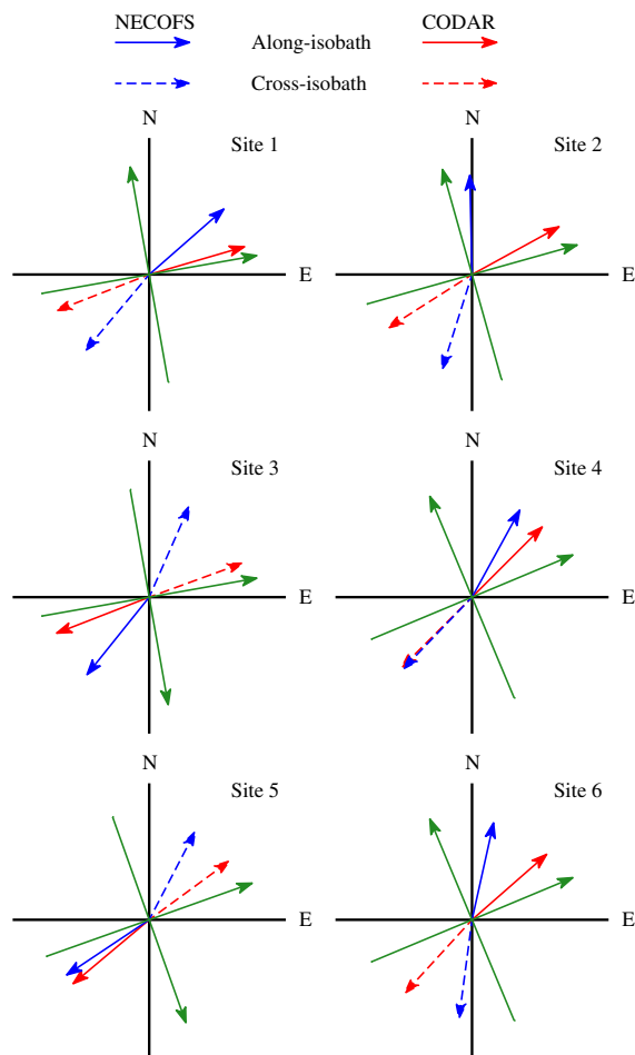
Fig. 16. The direction corresponding to the maximum correlation between wind stress and the along- and cross-isobath surface current at the six sites shown in Fig. 1. The along- and cross-isobath components are color coded as above. The green coordinates show the local along- and cross-isobath direction. (For interpretation of the references to color in this figure legend, the reader is referred to the web version of this article.)
