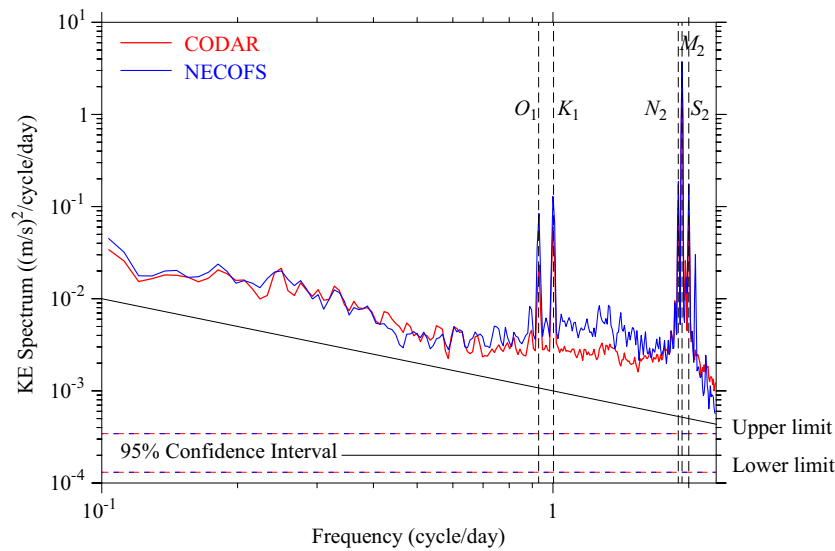
Fig. 4. Comparison of CODAR-derived and NECOFS-computed current kinetic energy spectral densities averaged over 4 sites (Fig. 2). The horizontal dash lines are the 95% confidence upper and lower limits (red: CODAR, blue: NECOFS). The vertical dashed lines mark the frequencies of M_2 , N_2 , S_2 , O_1 , and K_1 tidal constituents. (For interpretation of the references to color in this figure legend, the reader is referred to the web version of this article.)
