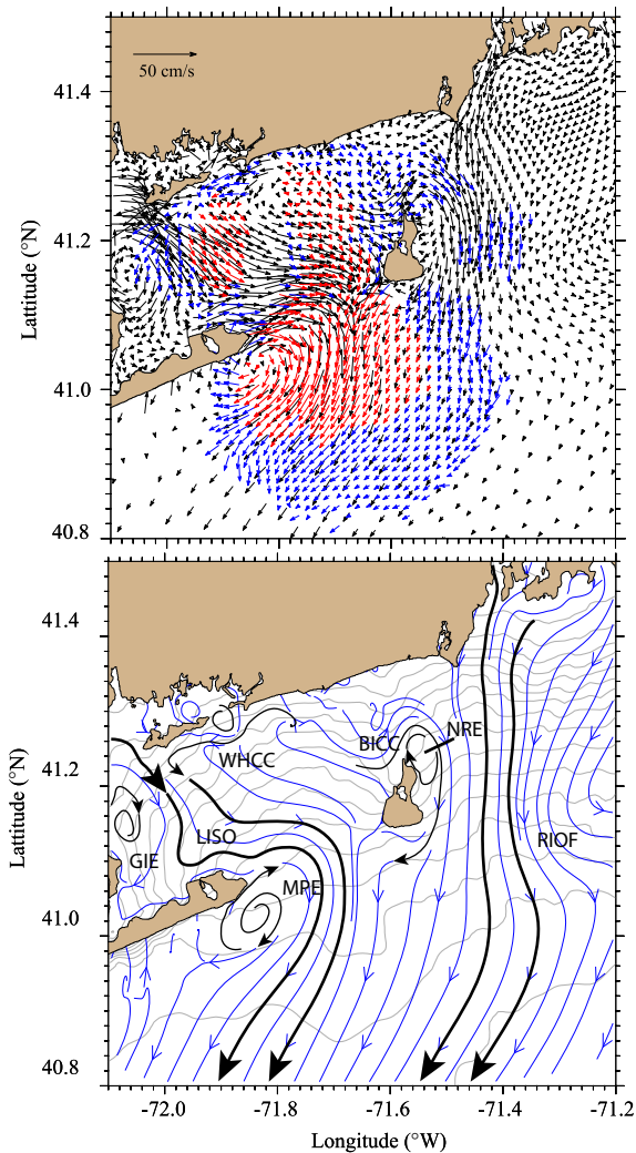
Fig. 8. Upper panel: comparisons of model-computed and CODAR-derived annual mean surface currents in Block Island Sound region. Black arrows: model-computed; red arrows: CODAR-derived at the selected grid points; blue arrows: CODAR-derived at all the grid points except the 334 selected. Lower panel: The gray contours are the potential function lines. Overlaid on the streamlines is a schematic outlining feature of the flow pattern: MPE is Montauk Point Eddy; GIE is Gardiners Island Eddy; LISO is Long Island Sound Outflow; NRE is North Reef Eddy; BICC is Block Island Clockwise Circulation; WHCC is Watch Hill Coastal Current; and RIOF is Rhode Island Offshore Flow. (For interpretation of the references to color in this figure legend, the reader is referred to the web version of this article.)
