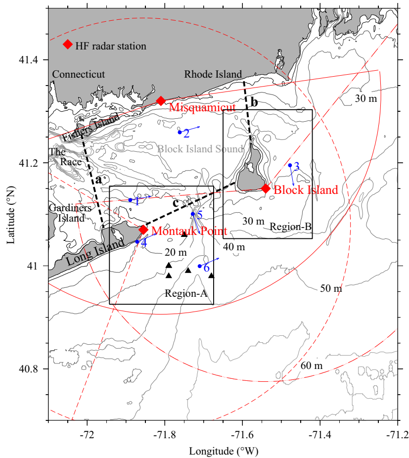
Fig. 1. The locations of three high frequency (HF) coastal ocean dynamics application radar (CODAR) stations at Montauk Point, Misquamicut and Block Island (red diamonds) and their nominal coverage areas (marked by red sectors). The black triangles indicate the ADCP locations. The blue dots indicate the locations of the six sites numbered 1–6 that were selected for the current–wind correlation analysis. The blue arrows show the along-isobath direction used to define the velocity components at these sites (cross-isobath is 90° counterclockwise from this direction). Dashed black lines are transects a, b, and c where the water cross-transect transports were calculated. The boxes labeled Region-A and Region-B are the areas where model-computed and CODAR-derived vorticities were compared. (For interpretation of the references to color in this figure legend, the reader is referred to the web version of this article.)
