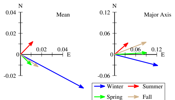
Fig. 15. Mean wind stress (left panel) and major principal axis (right panel) at the six sites in the four seasons. Units: N/m^2 . Note difference in scale.
