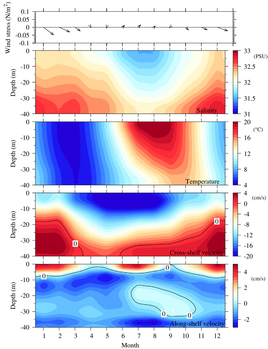
Fig. 21. Nine-year averaged wind stress, salinity, temperature profile at site 6, cross-shelf velocity profile (positive is onshore toward the north), along-shelf velocity profile (positive is along-shelf toward the west).
