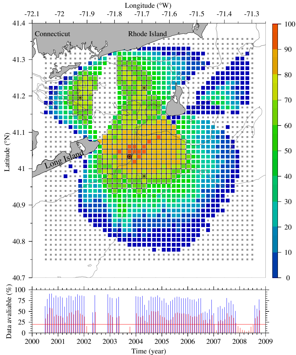
Fig. 2. The gridded CODAR data locations for a 46 \times 43 grid. In the upper panel, the colored squares show the percentage of the data available in each grid cell, the gray squares show no data available. The 334 sites with data availability greater than 60% and used for analysis are outlined in black. The black asterisks mark the four locations selected for the spectral analysis. The lower panel shows the percentage of hourly data available in each month; the blue vertical lines are for the 334 grid points, and the red vertical lines are for the 1147 grid points with data, and the red horizontal line at 20% is the lower limit for 'system on' monthly data. (For interpretation of the references to color in this figure legend, the reader is referred to the web version of this article.)
