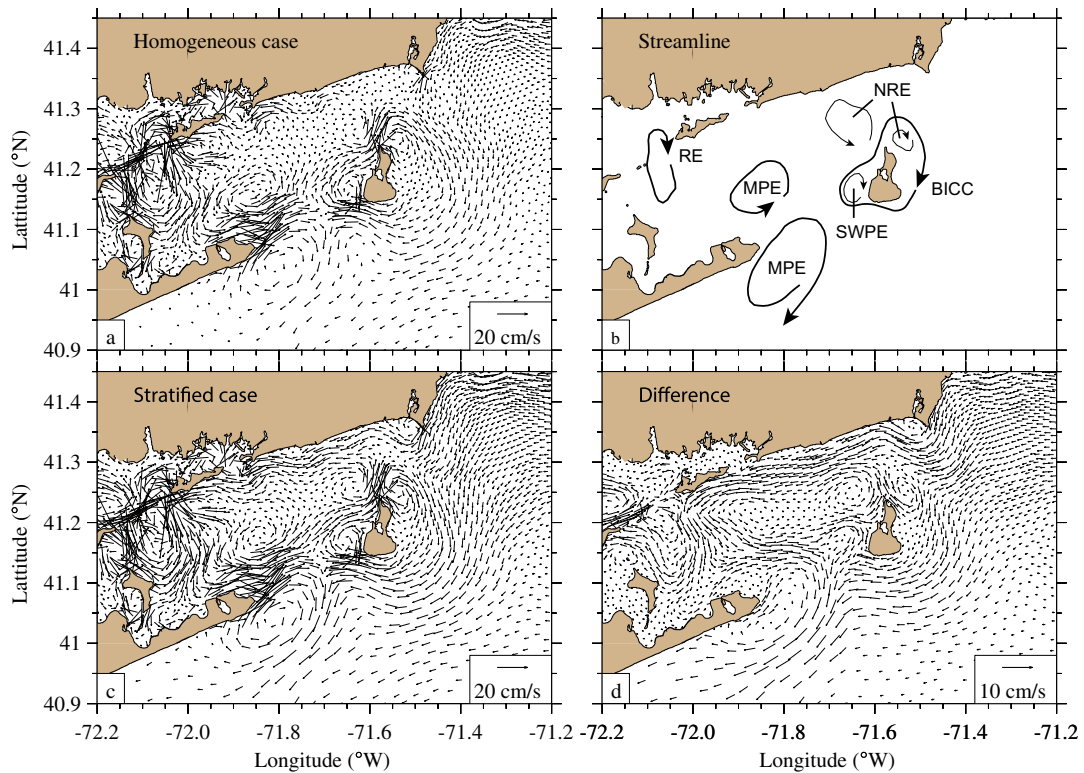
Fig. 19. Distribution of the depth averaged tidal residual flow in (a) homogeneous conditions, (b) its corresponding schematic diagram, (c) tidal residual flow in summertime stratified conditions, and (d) their difference (stratified minus homogeneous cases). In (b), RE is Race Eddy; MPE is Montauk Point Eddy; NRE is North Reef Eddy; BICC is Block Island Clockwise Circulation; and SWPE is Southwest Point Eddy.
