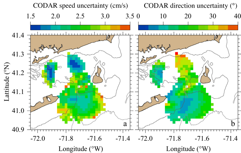
Fig. 3. The distribution of the CODAR data measurement uncertainty averaged over the total hourly record at the 334 grid points. (a) Speed (cm/s) and (b) direction ( ^{\circ} ).
