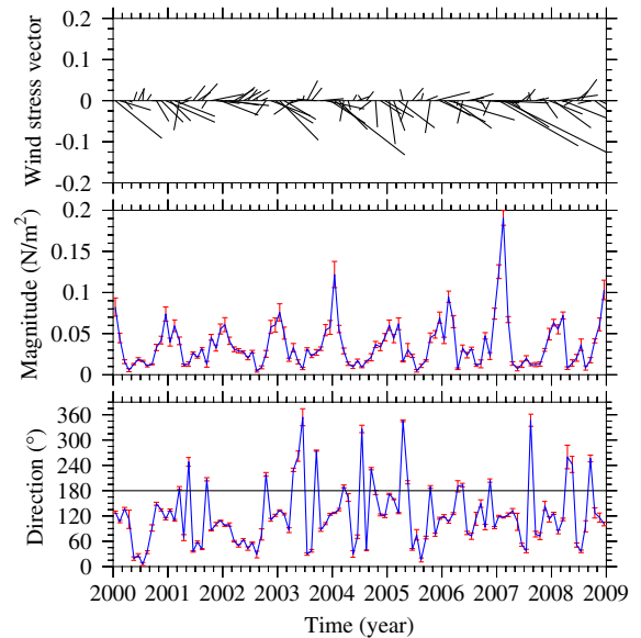
Fig. 14. Time series of the monthly-mean surface wind stress vector (upper panel), its magnitude (middle panel) and direction (lower panel) averaged over sites 1–6 over the period of 2000–2008. The vertical red line segment indicates the standard deviation over the six sites for each month. (For interpretation of the references to color in this figure legend, the reader is referred to the web version of this article.)
