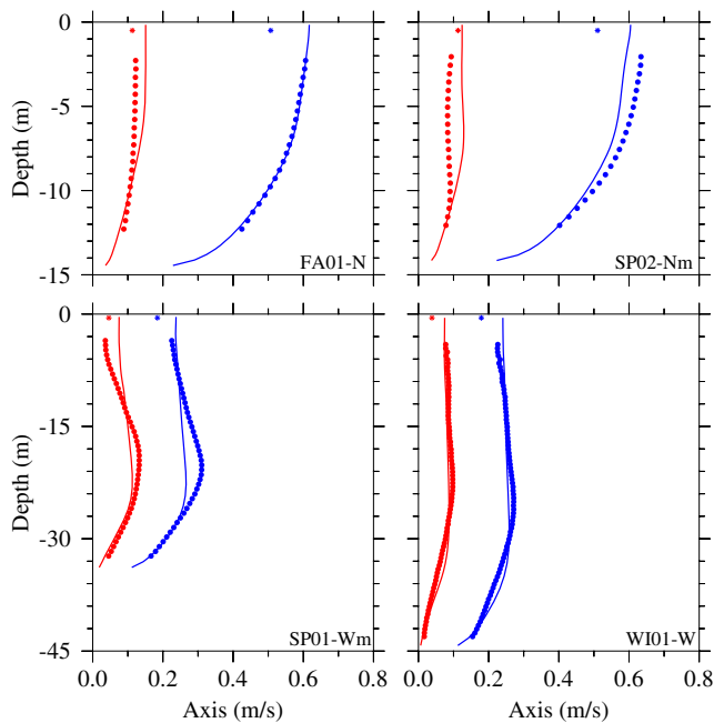
Fig. 17. Vertical profile of the ADCP-derived (dots), CODAR-derived (asterisks) and model-computed (solid lines) for major axis (m/s, blue color) and minor axis (m/s, red color), based on ADCP-derived and model-computed M 2 tidal currents at 4 stations: FA01-N, SP02-Nm, SP01-Wm and WI01-W. (For interpretation of the references to color in this figure legend, the reader is referred to the web version of this article.)
