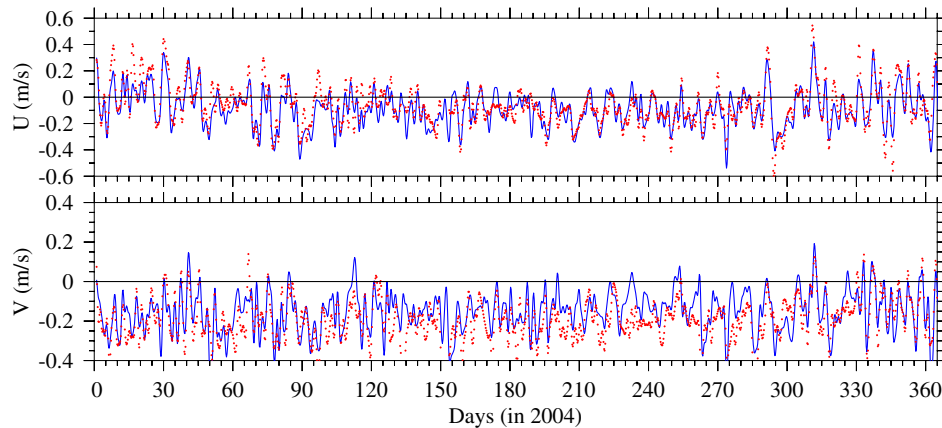
Fig. 7. Subtidal current comparison between CODAR (red dots) and model (blue line) in 2004 at the circled asterisks CODAR station in Fig. 2. (For interpretation of the references to color in this figure legend, the reader is referred to the web version of this article.)
